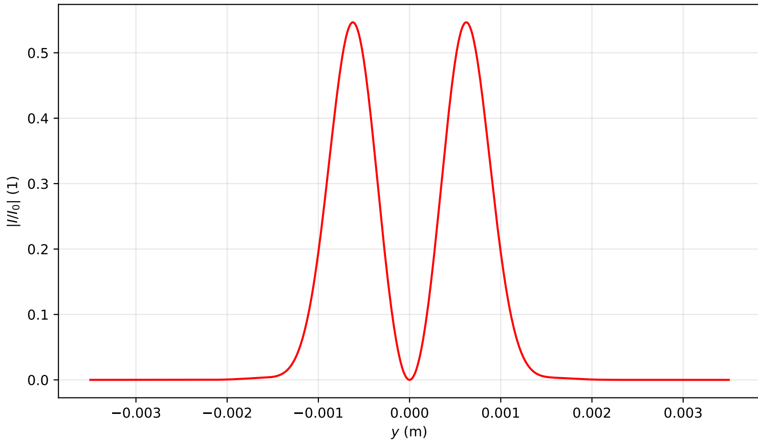
Intensity profile I(x=0, y, z=1.353)/I_0 , \text{Pin}=2.0\text{Pcr} , artificial time
